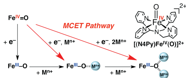
Scheme 1. MCET of [(N4Py)Fe IV (O)] 2+
