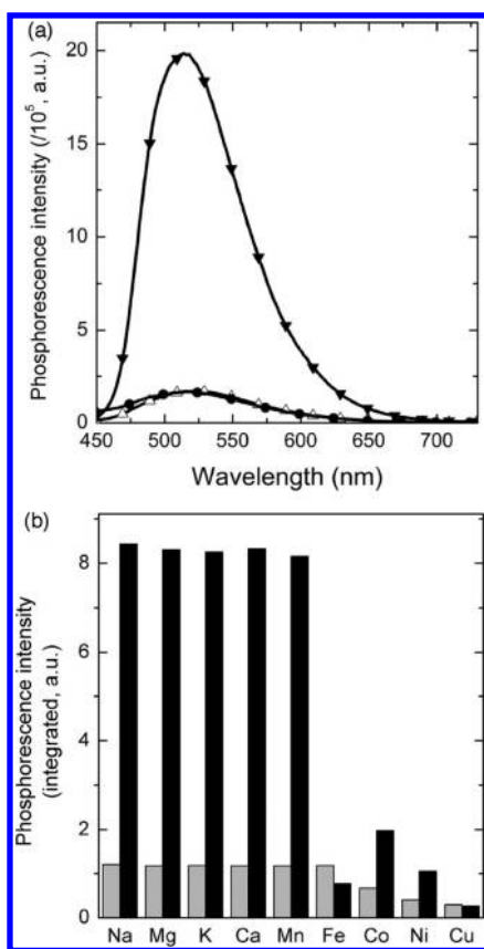
Figure 5. (a) Phosphorescence spectra of ZIrF showing reversible binding with zinc ions: \Delta , zinc-free solution; \nabla , in the presence of zinc ion (1 equiv); \bullet , after subsequent addition of TPEN (5 equiv). (b) Phosphorescent zinc selectivity of ZIrF: gray bars, in the presence of metal ions; black bars, after subsequent addition of \text{ZnCl}_2 (1 equiv). \text{Na}^+ , \text{Mg}^{2+} , \text{K}^+ , and \text{Ca}^{2+} ions are 100 equiv. Other divalent metal ions are 1 equiv. Chloride salts were used. Conditions: 10 \mu\text{M} ZIrF in air-equilibrated pH 7.0 buffer (25 mM PIPES), \lambda_{\text{ex}} = 340 \text{ nm} .
