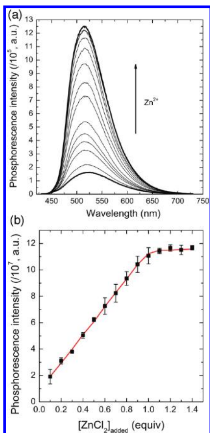
Figure 4. (a) Change in phosphorescence spectrum with varying total zinc concentration. (b) Corresponding phosphorescence titration isotherm. The red solid line is a theoretical fit. Refer to text for the theoretical model. Conditions: 10 \mu\text{M} ZIrF in air-equilibrated pH 7.0 buffer (25 mM PIPES), \lambda_{\text{ex}} = 340 nm.
