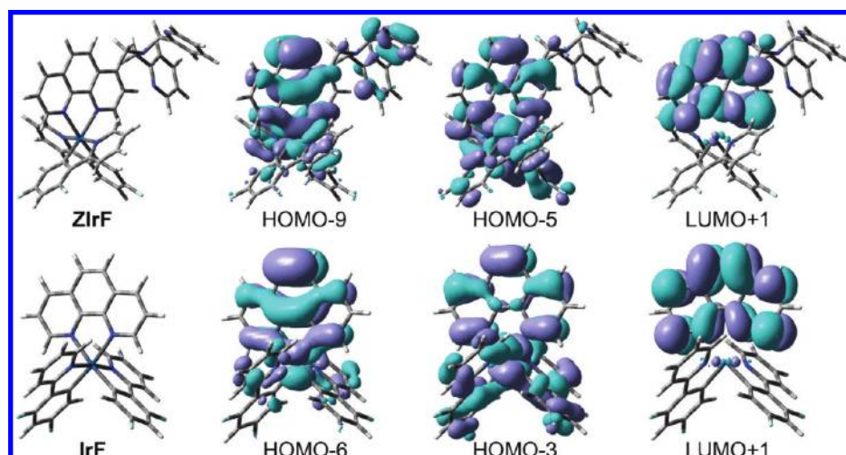
Figure 1. Calculated geometry and isosurface plot ( 0.04 e \text{ \AA}^{-3} ) of molecular orbitals that participate in the lowest energy triplet transitions of ZIrF and IrF, as obtained from Gaussian 03.
